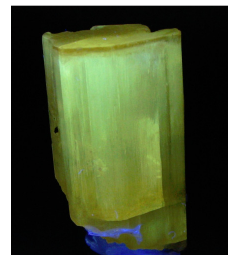
Phosgenite - Under SW UV
